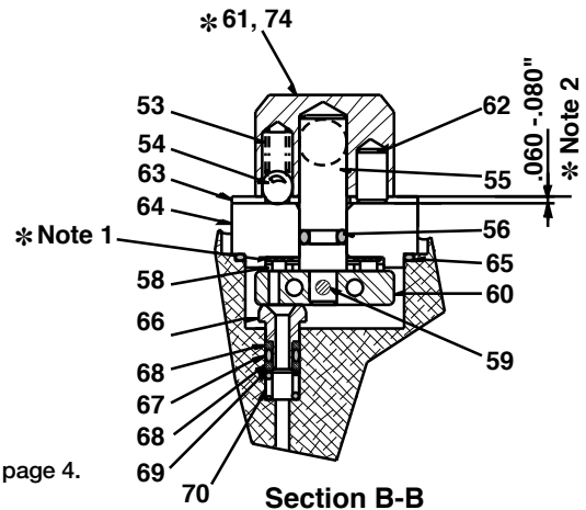
Fig. 3, P-842 Only - Section B-B
