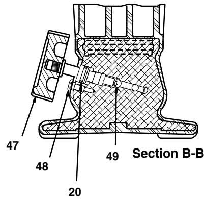
Fig. 2, P-802 Only - Section B-B
