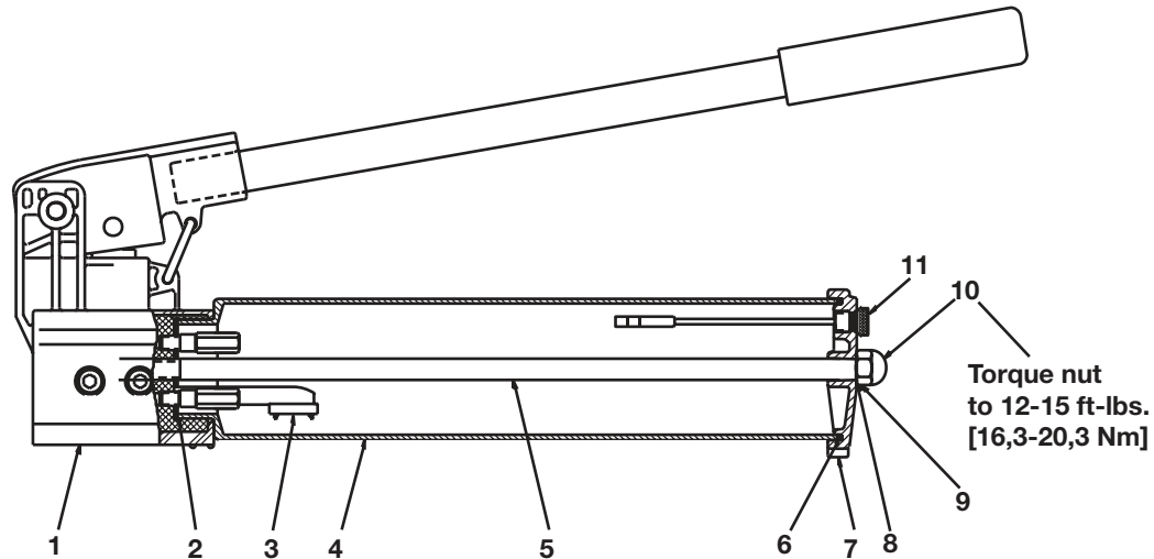
Figure 1, Pump Assembly
