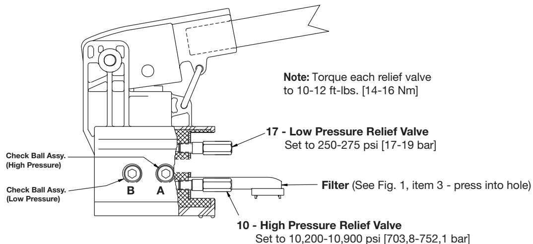
Figure 2, Pumping Unit Assembly (See parts list on page 2)
