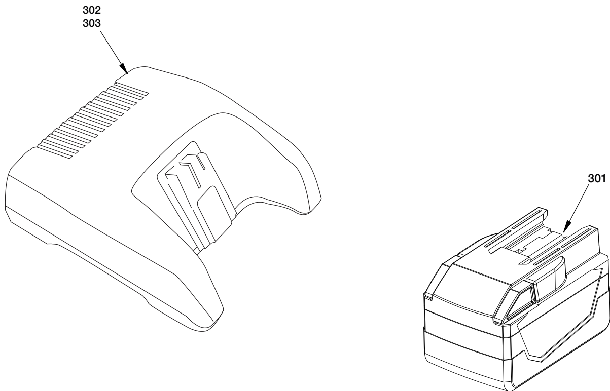
Fig. 15, Battery & Charger
