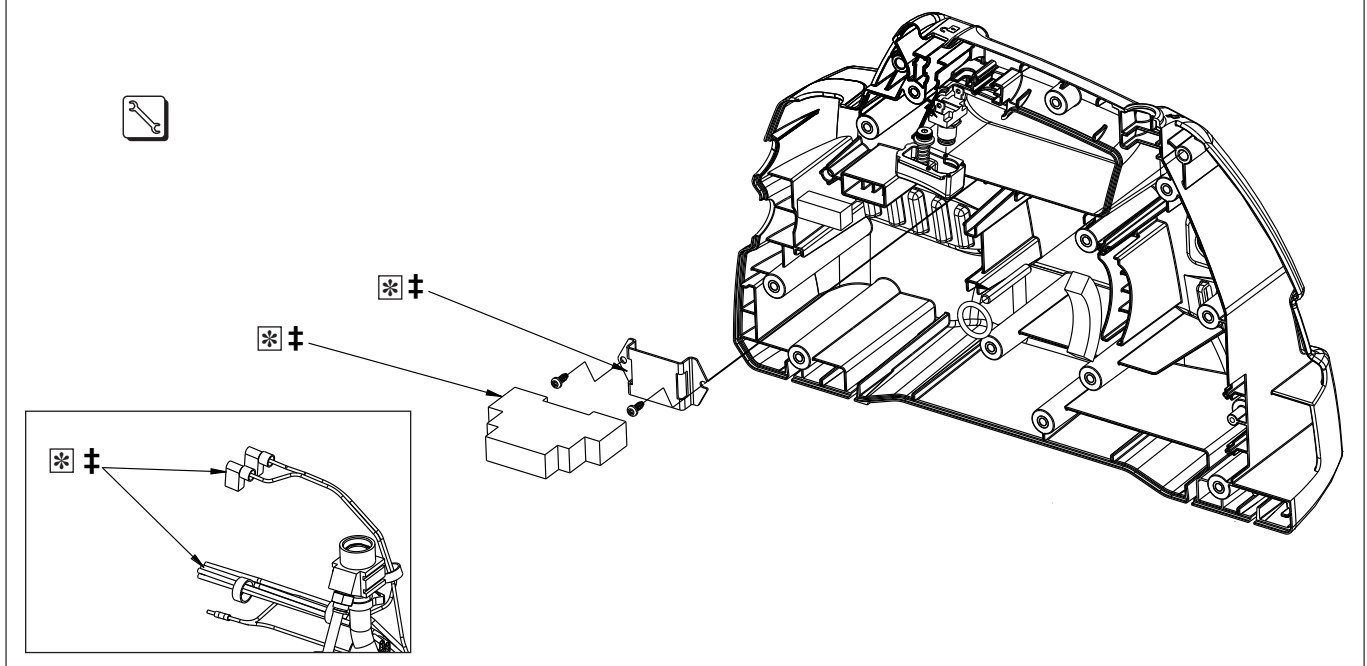
Fig. 3B, Electrical Components, Old Style (originally installed on pumps with date codes "A" and "B")
