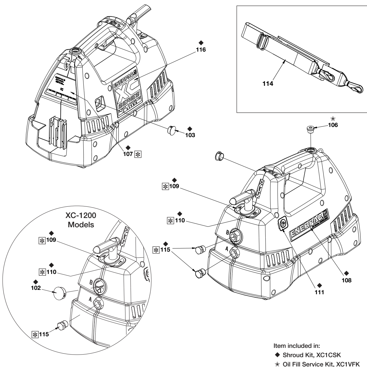
Fig. 1, Decals, Plugs, Caps & Shoulder Strap
