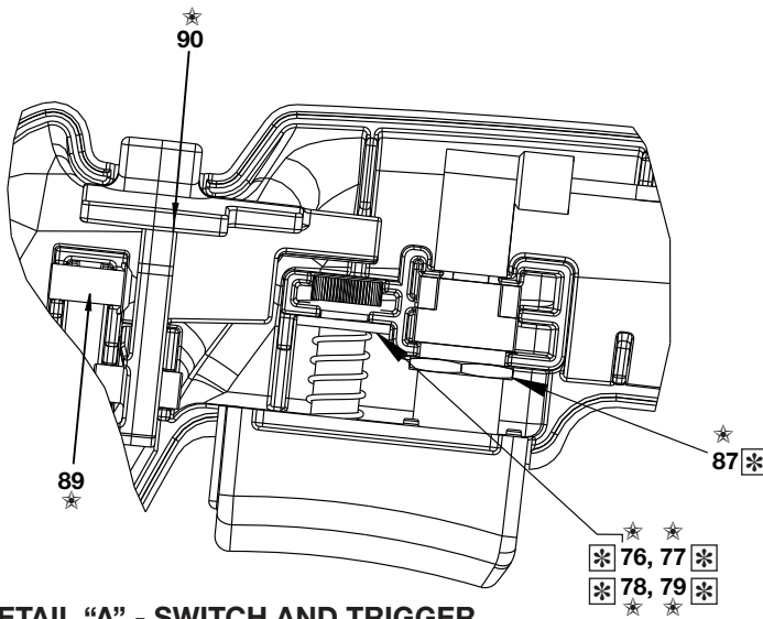
DETAIL "A" - SWITCH AND TRIGGER
