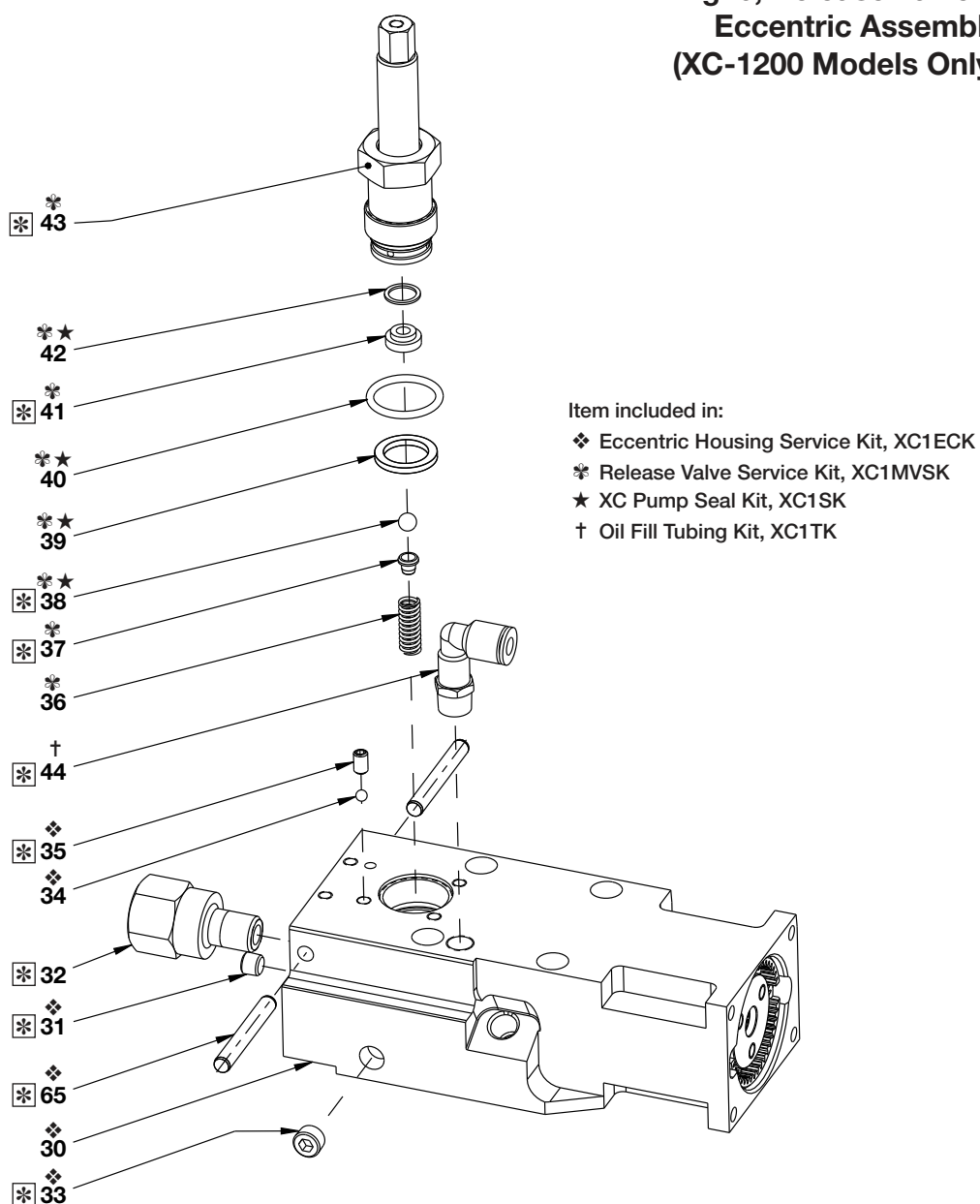
Repair Parts List, Fig. 6
