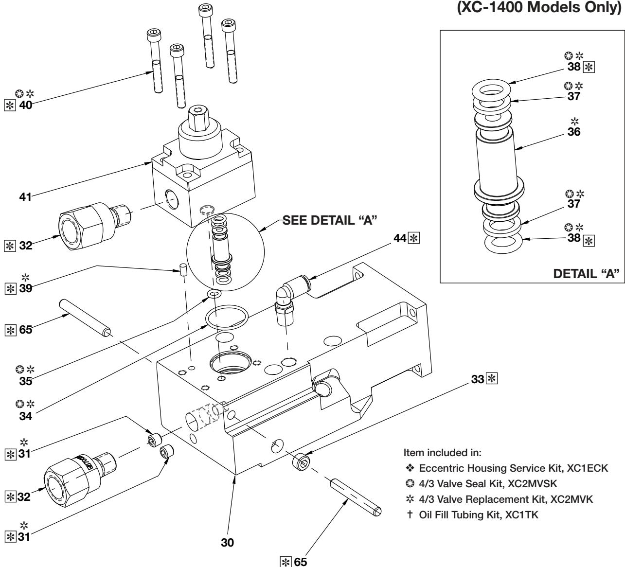
Repair Parts List, Fig. 8
