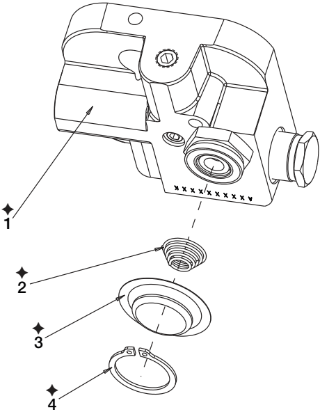
Fig. 13, Pump Assembly
