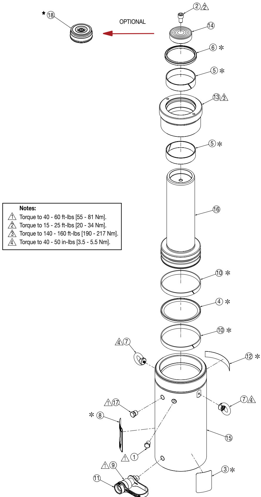
Figure 4, Exploded View - Model HCG-100 Tall
