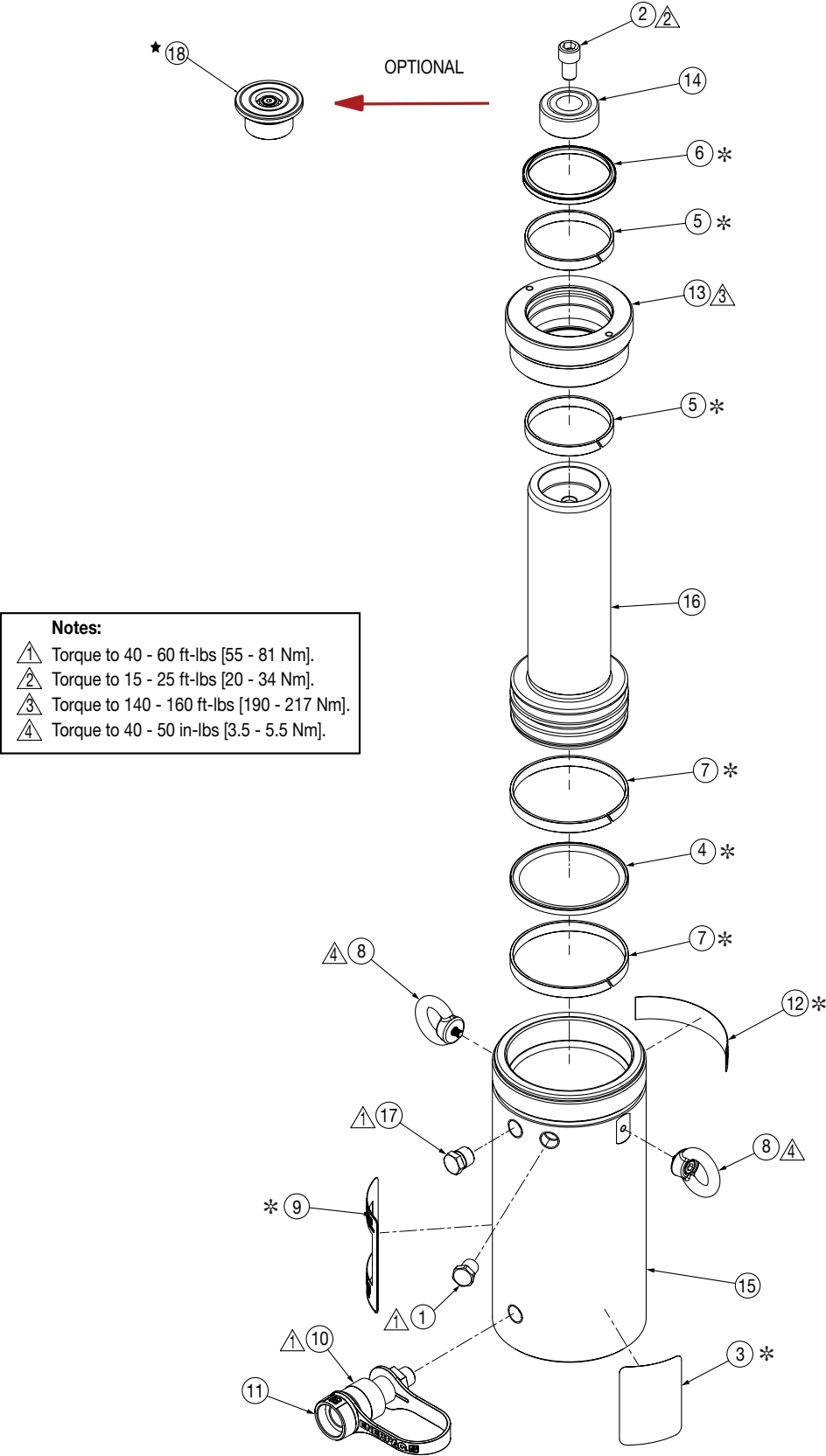
Figure 1, Exploded View - Model HCG-50 Short
