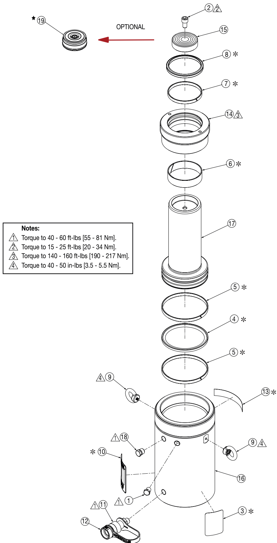
Figure 3, Exploded View - Model HCG-100 Short
