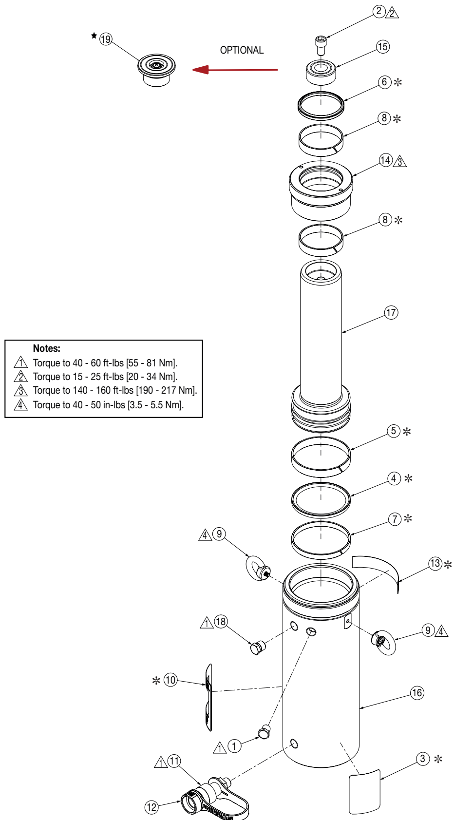
Figure 2, Exploded View - Model HCG-50 Tall
