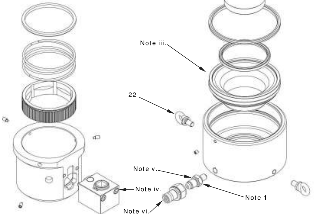
Figure 2, Exploded View, PGT Single Stage Tensioner with Lift Support
