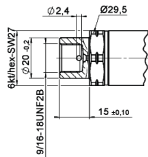
HDA 4XBX Einschraubloch/ Screw plug hole 9/16-18 UNF2B (F250C, Autoclave)
