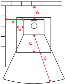
Recommended distances to non-combustibles
