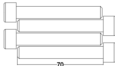
70 NO.26 M10x70(4)
