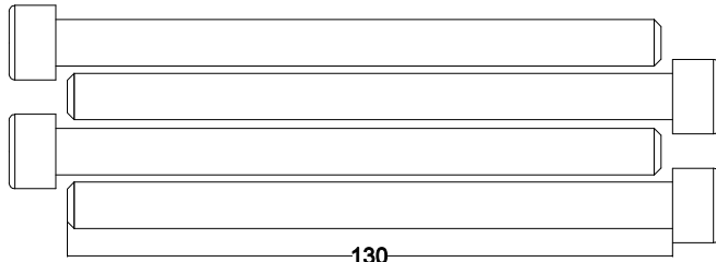
130 NO.24 M10x130(4)
