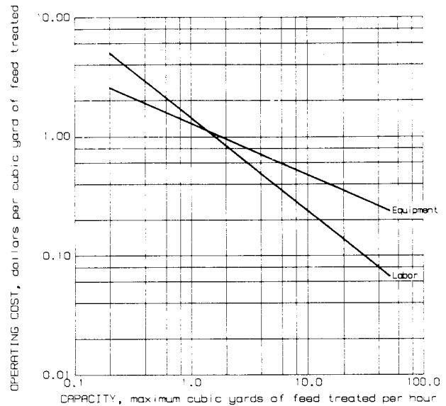
Processing operating costs - Table concentrators
