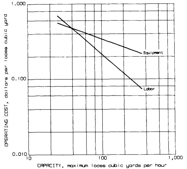
Mining operating costs - Draglines
