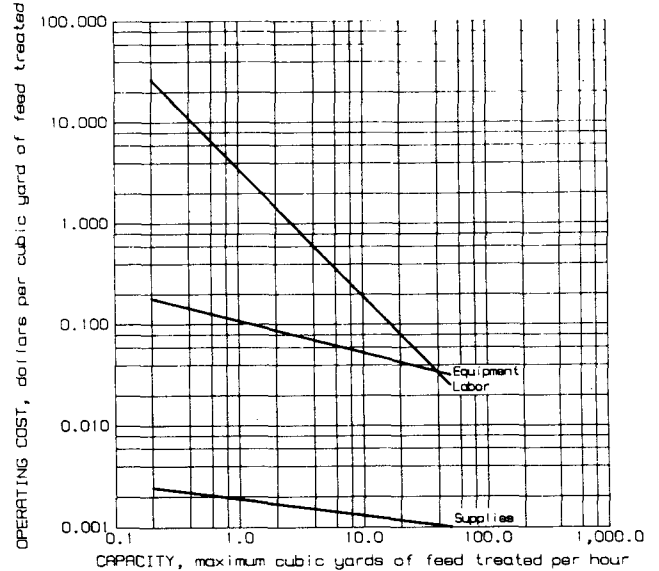
Processing operating costs - Jig concentrators
