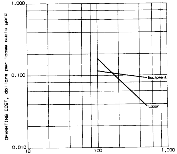
Processing operating costs - Tailings removal - Scrapers
