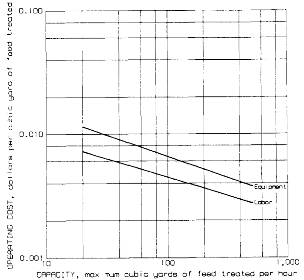
Processing operating costs - Feed hoppers
