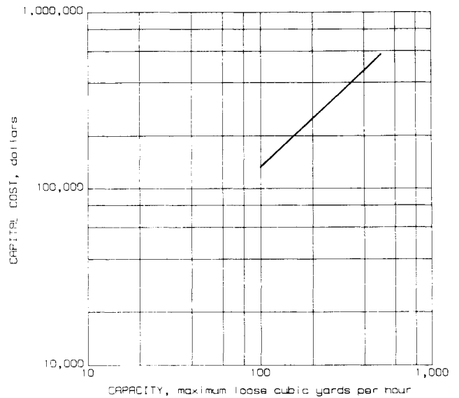
Mine equipment capital costs - Scrapers
