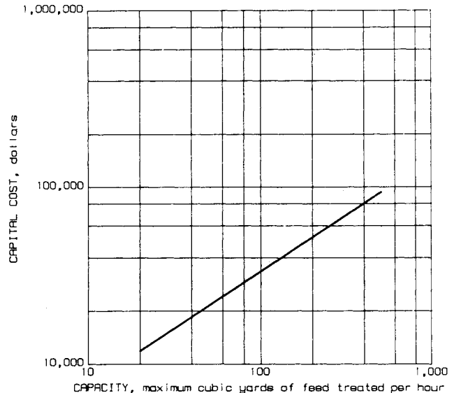
Processing equipment capital costs - Vibrating screens
