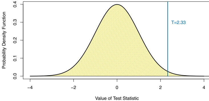
FIGURE 13.1. The density function for the N(0, 1) distribution, with the vertical line indicating a value of 2.33. 1% of the area under the curve falls to the right of the vertical line, so there is only a 2% chance of observing a N(0, 1) value that is greater than 2.33 or less than -2.33 . Therefore, if a test statistic has a N(0, 1) null distribution, then an observed test statistic of T = 2.33 leads to a p -value of 0.02.
