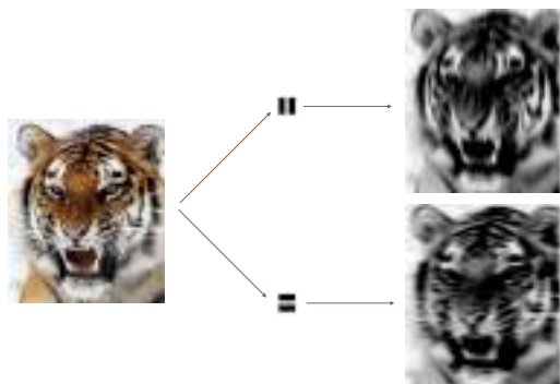
FIGURE 10.7. Convolution filters find local features in an image, such as edges and small shapes. We begin with the image of the tiger shown on the left, and apply the two small convolution filters in the middle. The convolved images highlight areas in the original image where details similar to the filters are found. Specifically, the top convolved image highlights the tiger’s vertical stripes, whereas the bottom convolved image highlights the tiger’s horizontal stripes. We can think of the original image as the input layer in a convolutional neural network, and the convolved images as the units in the first hidden layer.
