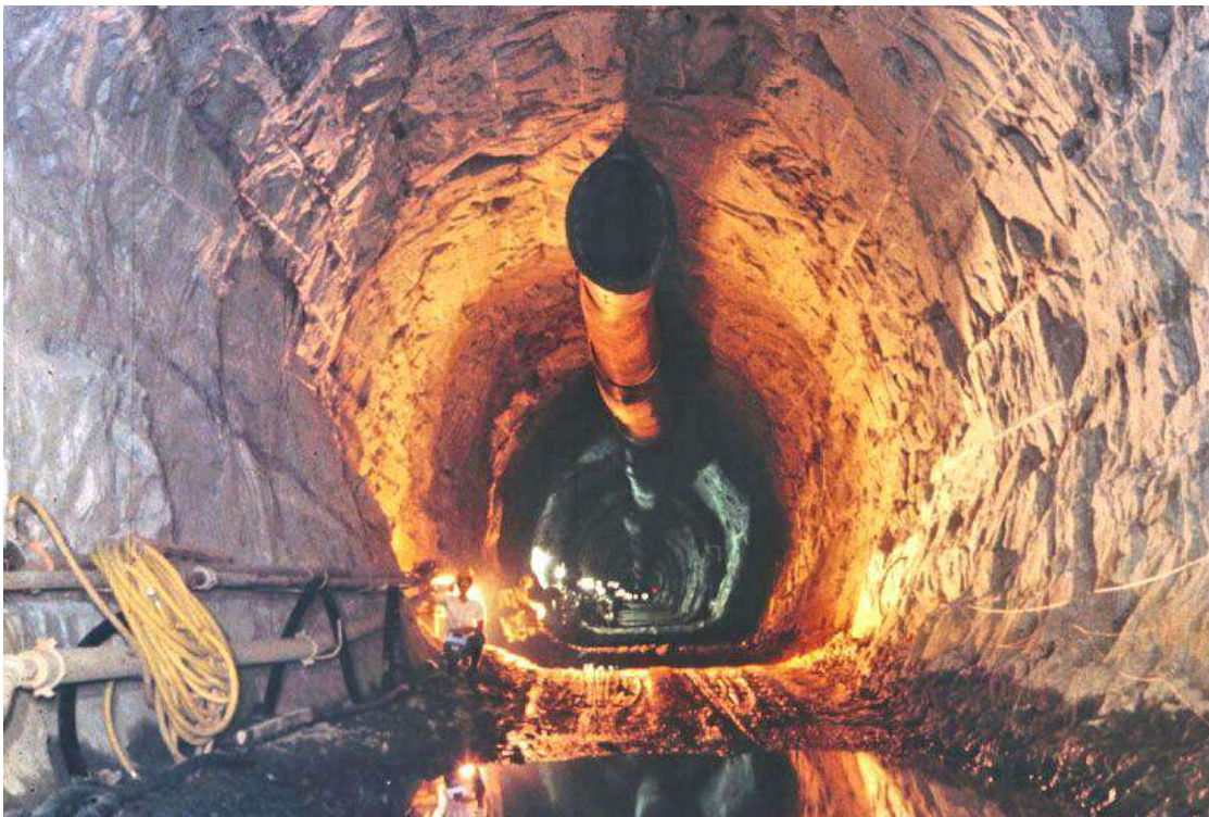
Figure 1.11: An example of good blasting in a tunnel.
