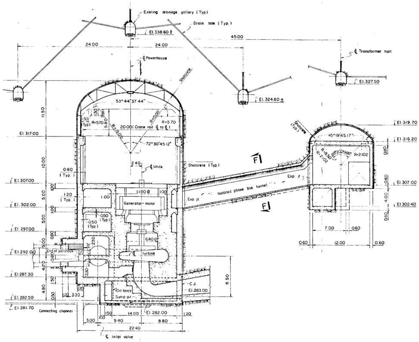
Figure 11: Final layout of Mingtan powerhouse cavern and transformer gallery.
