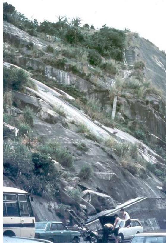
Figure 4: The failure surface defined by a sheet joint surface on which a small slide occurred during blasting of the original cut slope for the Sau Mau Ping Road. The potentially unstable slope under consideration is visible in the background.
