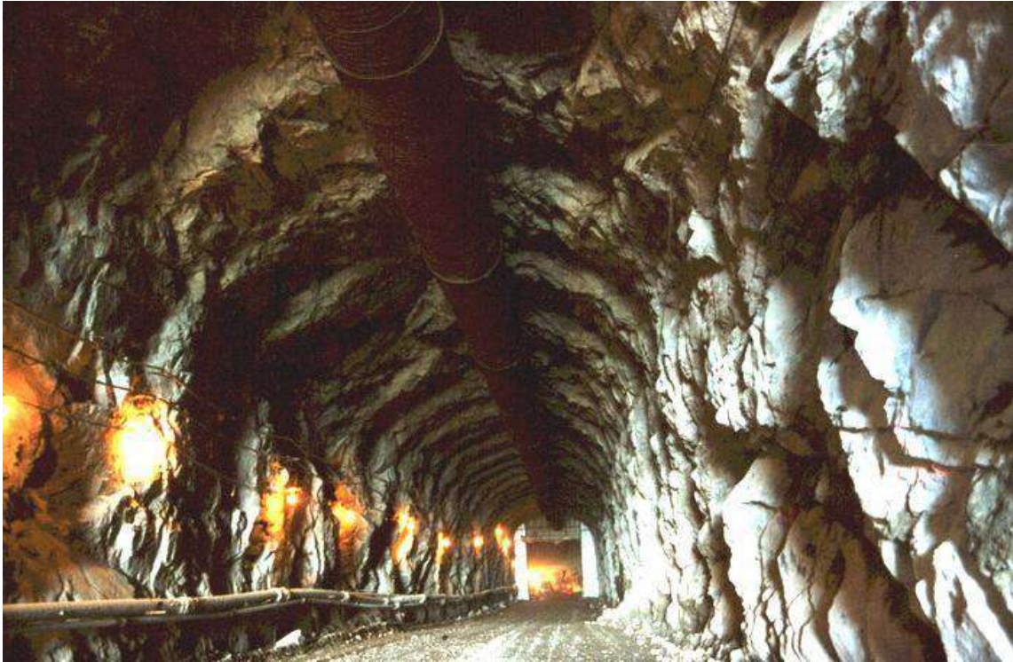
Figure 1.10: An example of poor blasting in a tunnel.
