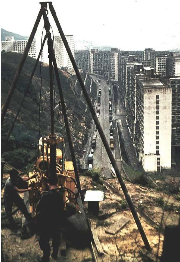
Figure 11: Drilling vertical diamond core holes into the Sau Mau Ping slope. These holes were used for geotechnical investigation purposes and also for the installation of piezometers in the rock mass.
