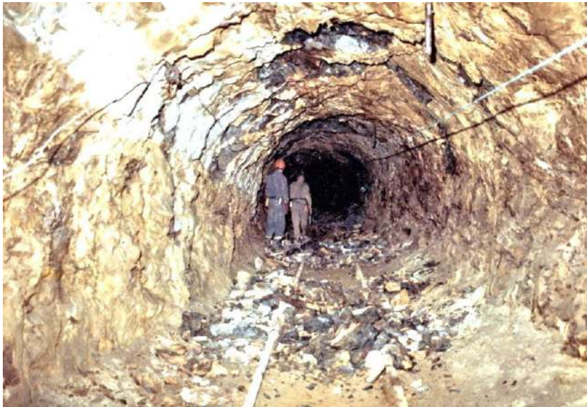
Figure 5: Ravelling of small wedges in a closely jointed rock mass. Shotcrete can provide effective support in such rock masses
