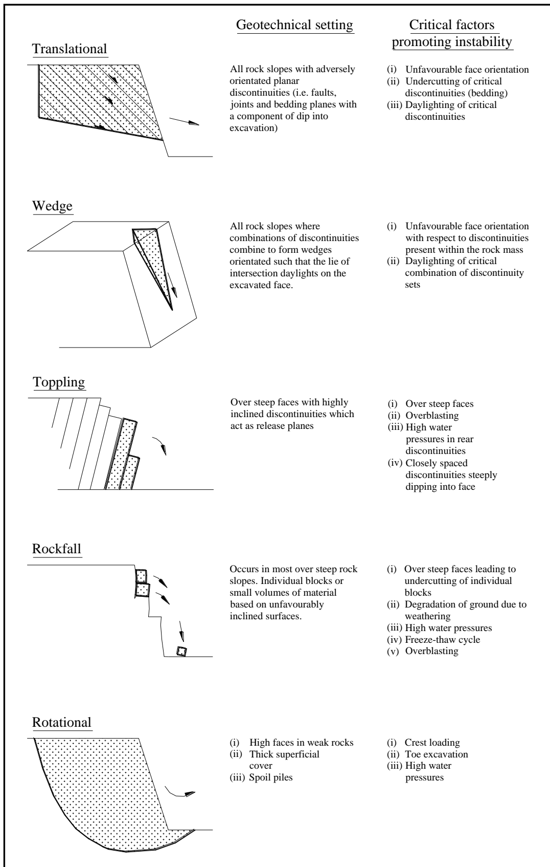
Figure 3 – Typical modes of failure in slopes
