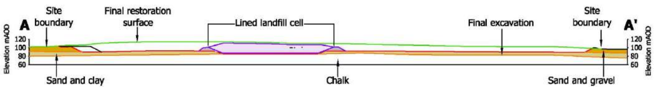
Figure 4-7 Example of a final excavation/restoration design for a sand and gravel operation
