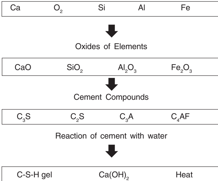
Fig-2 Reaction of cement with water
