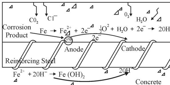
Fig-2 Electro-chemical Process of Corrosion
