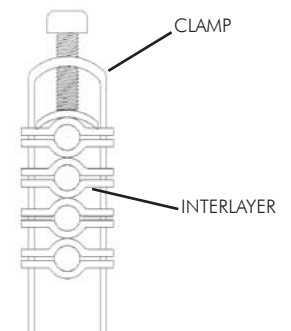
Example of standard clamp for 4 cables
