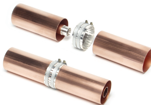
Unflange coupling kit assembly
