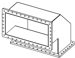
Example of E-bend design
