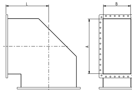
Example of H-bend design
