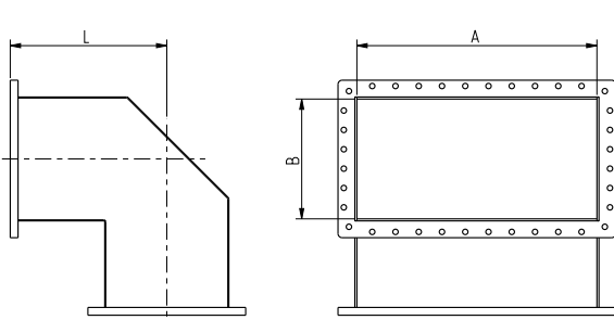
Example of E-bend design
