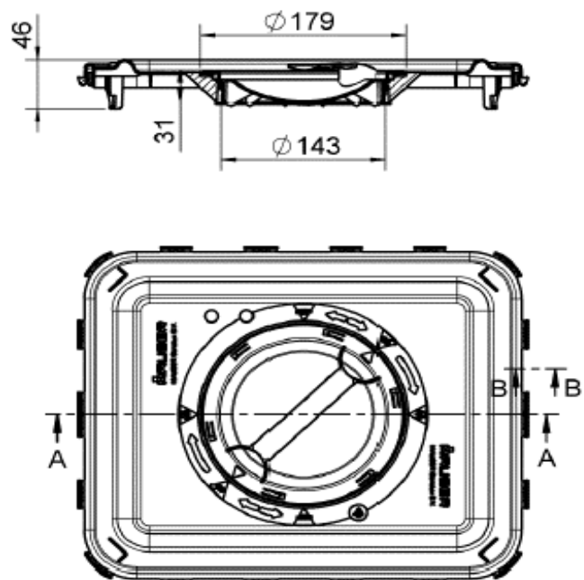
SECTIONAL VIEW A-A
