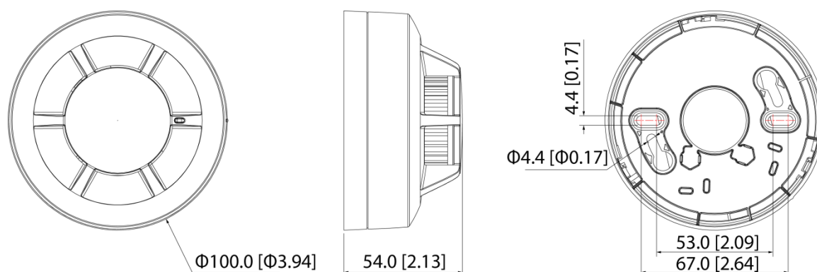
Figure 1-1 Dimension [mm (inch)]
