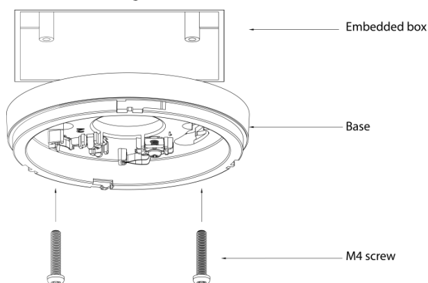
Figure 3-1 Installation (1)
