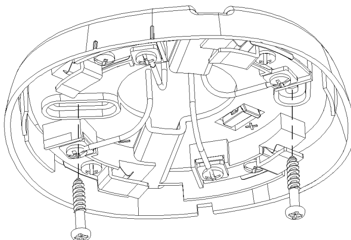
Figure 3-9 Installation (4)
