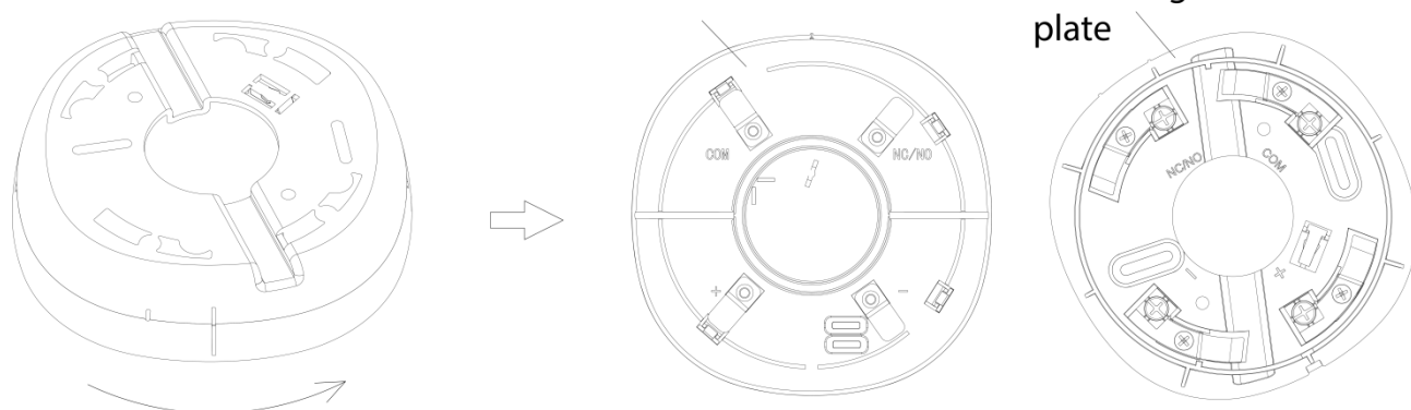
Figure 3-4 Installation (1) detector
