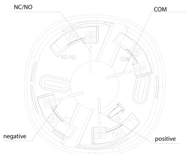
Figure 3-6 Installation (3)
