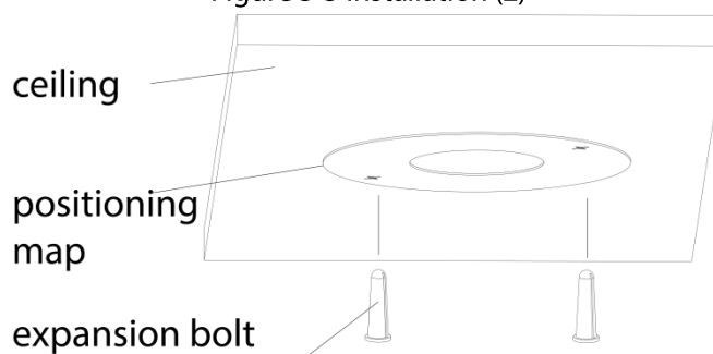
Figure 3-5 Installation (2)
