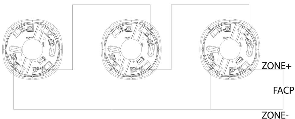
Figure 3-7 Wiring (1)
