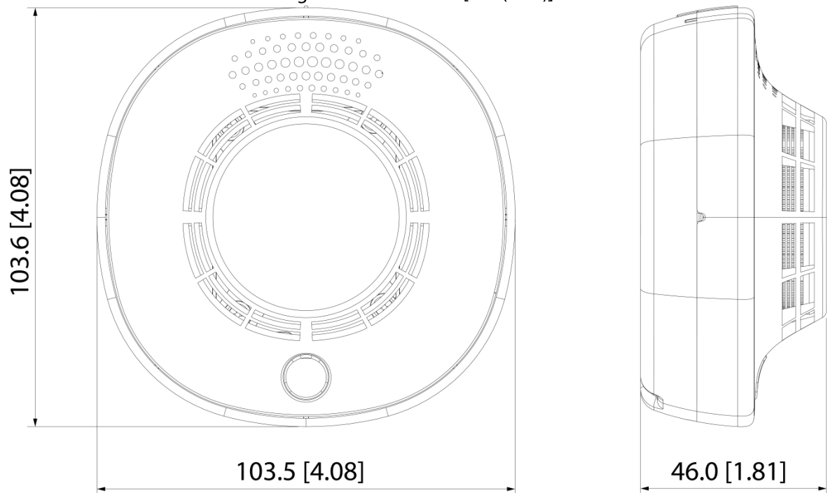
Figure 1-1 Dimension [mm(inch)]
