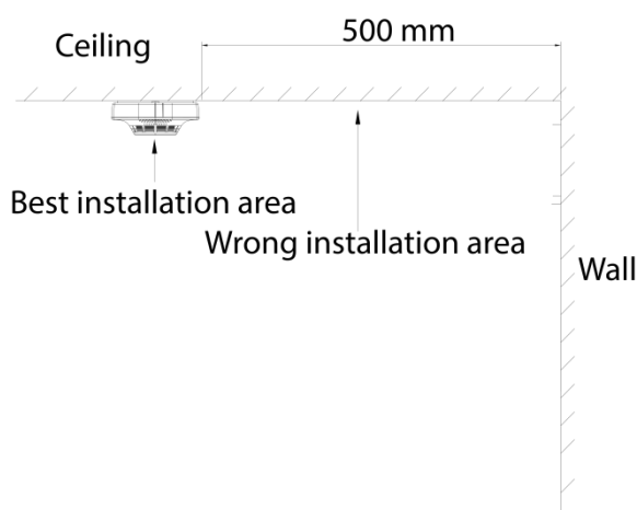
Figure 3-2 Installation position (1)
