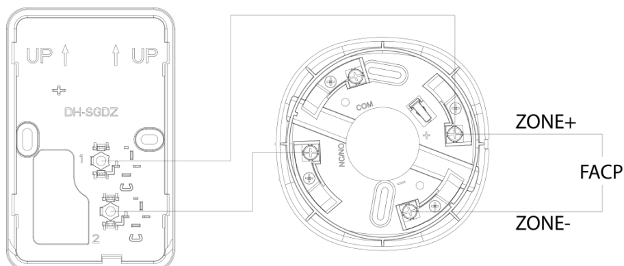
Figure 3-8 Wiring (2)
