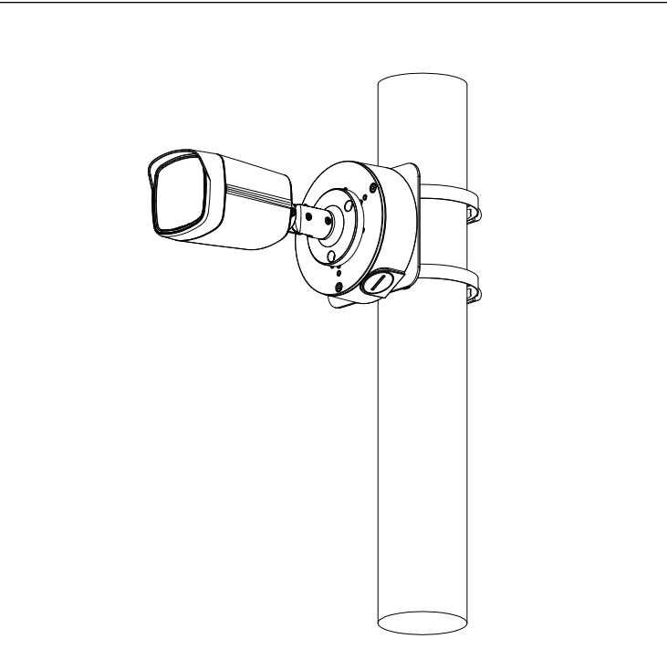
Pole Mount(Vertical)
