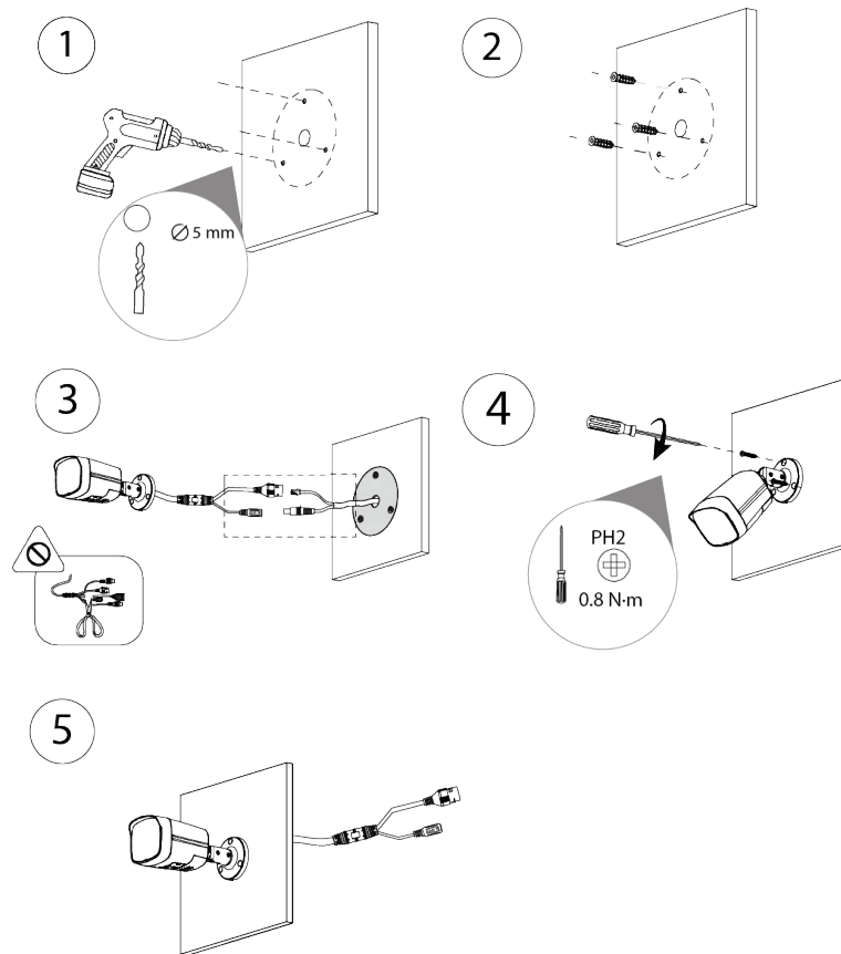
Figure 3-4 Cable going through the mounting surface
