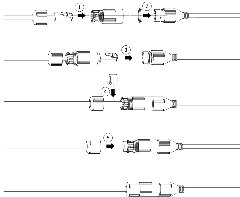
Figure 3-5 Install the waterproof connector
