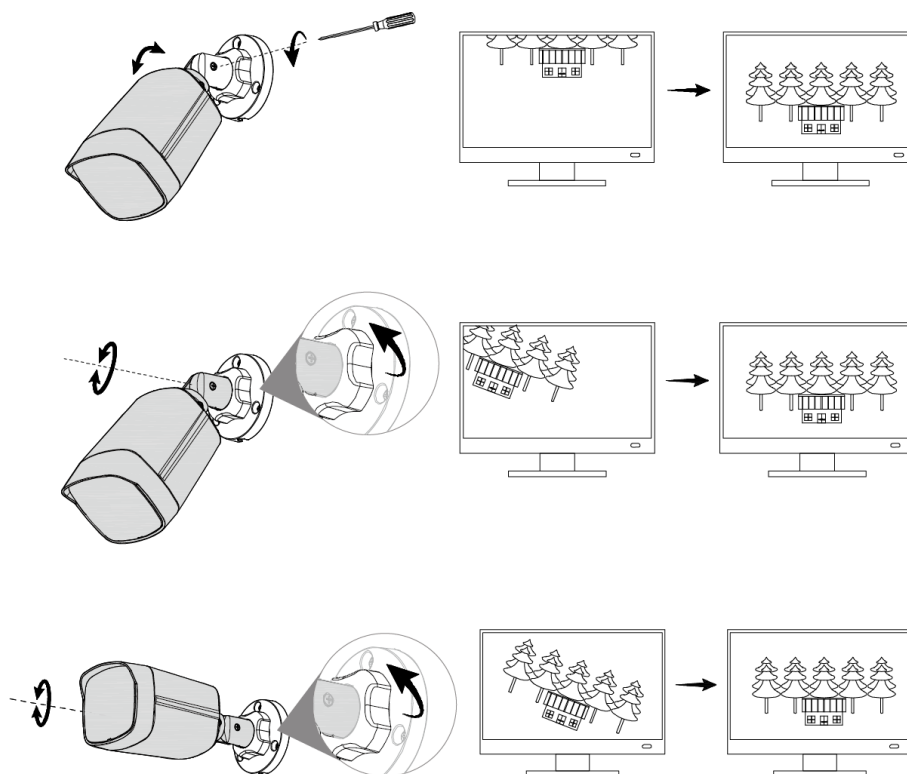
Figure 3-6 Adjust the lens angle
