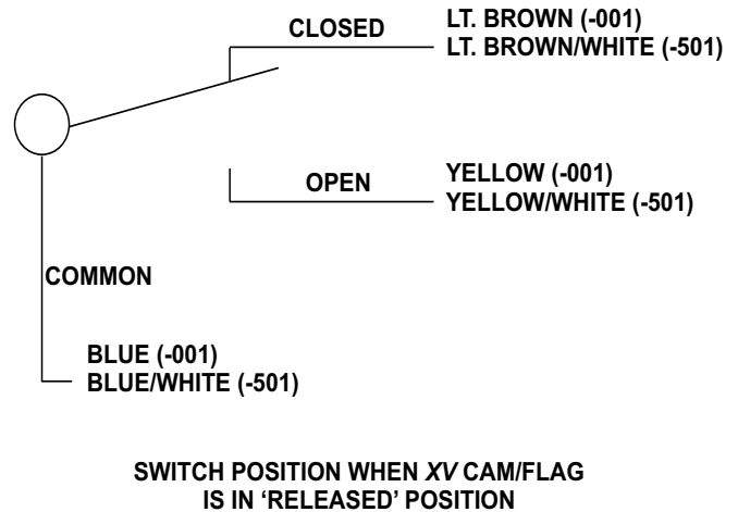
Figure 2. Microswitch in Released Position
