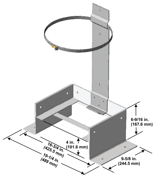
SHELF BRACKET ATTACHED TO FLOOR MOUNT BRACKET
