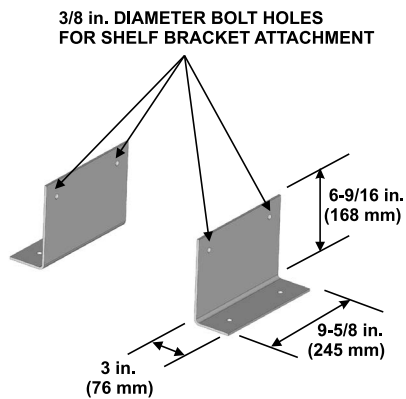
FLOOR MOUNT BRACKET KIT
