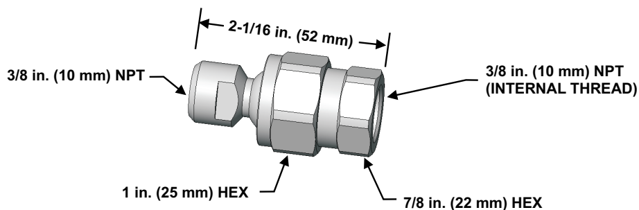
Figure 3. Nozzle Swivel Adapter
