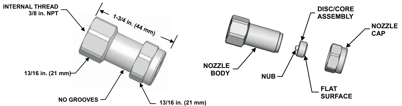
Figure 2. LPR Nozzle Dimensions and Assembly
