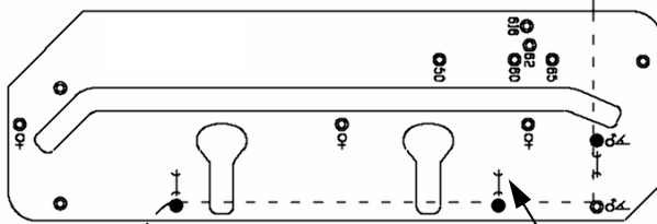
DIAGRAM D MALE BOLT RECESS — WORKTOP FACE DOWN.
