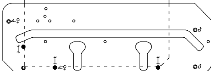
DIAGRAM D MALE BOLT RECESS — WORKTOP FACE DOWN.
