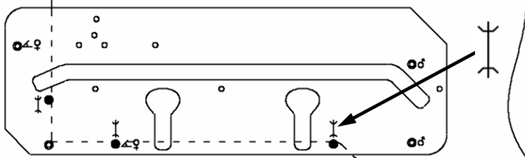
DIAGRAM D MALE BOLT RECESS— WORKTOP FACE DOWN.
