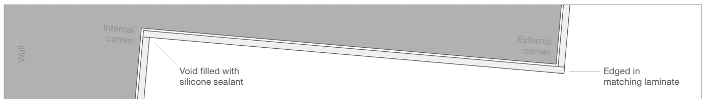
Fig 3: Internal/External Corner Detail
