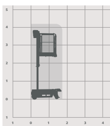
Working Envelope
