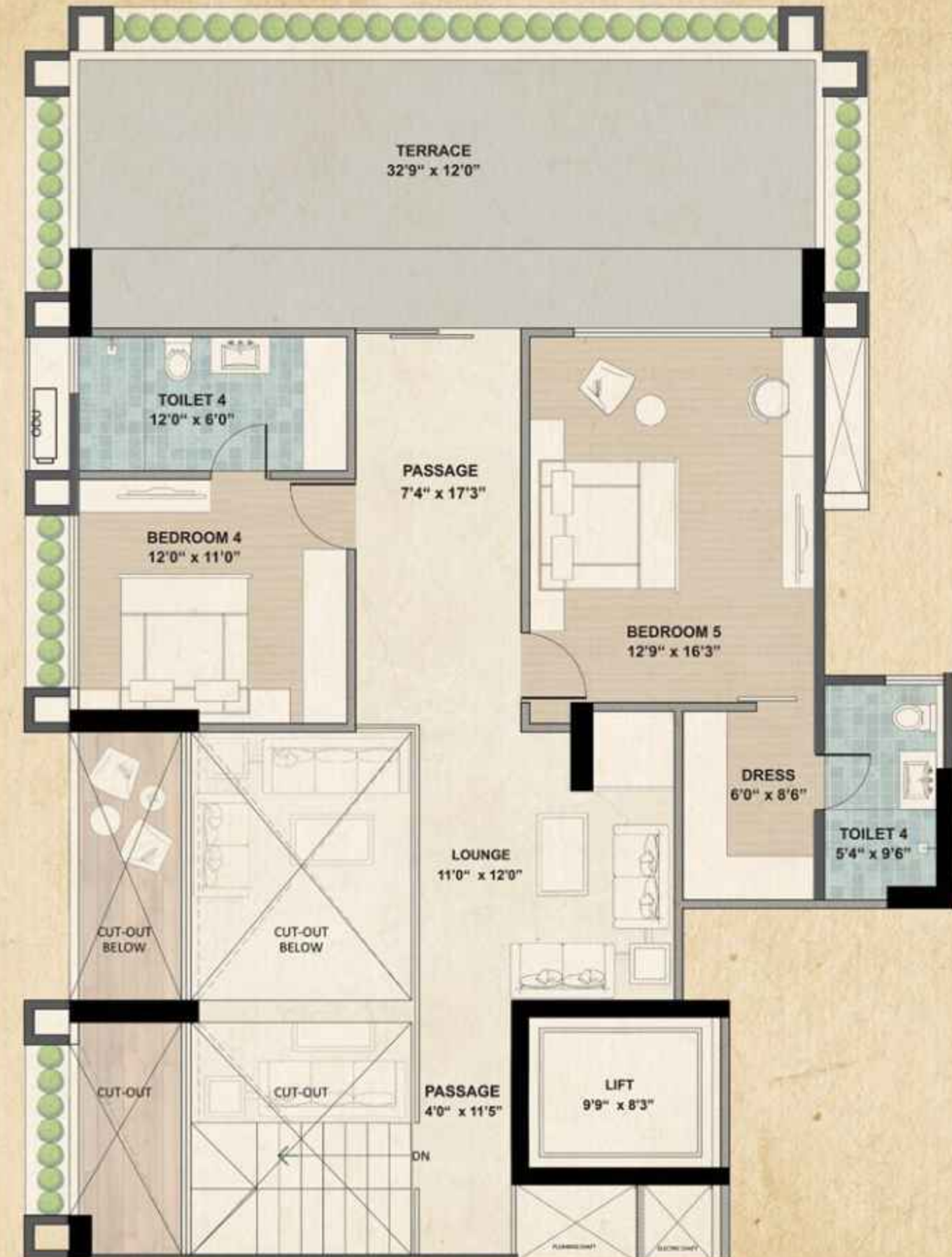
UPPER LEVEL
