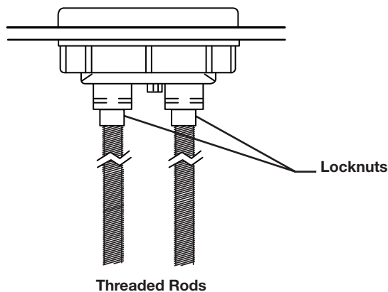
Threaded Rods
