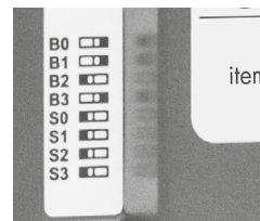
S Bank DIP Switch Location
