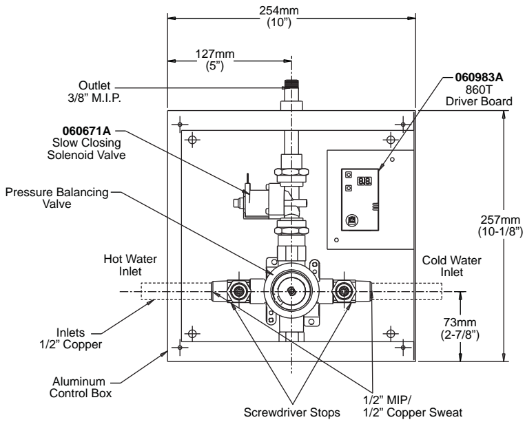
Fig. 6 Control Box #7
