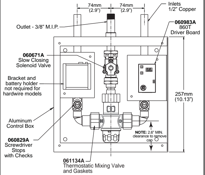
Fig. 7 Control Box #8
