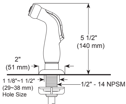
RP101326▲ Spray, Hose Assembly & Spray Support
