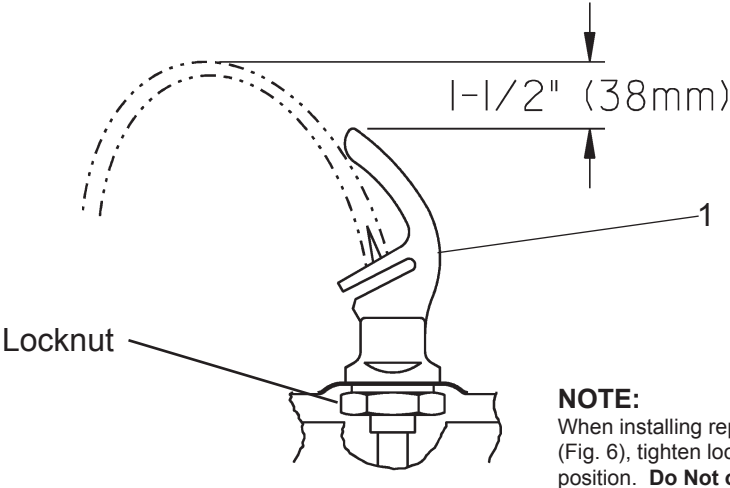
Figure 6 - Bubbler Detail
