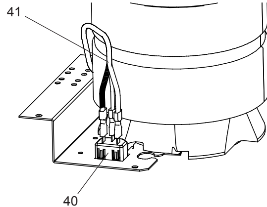
Fig. 15 220V Detail
