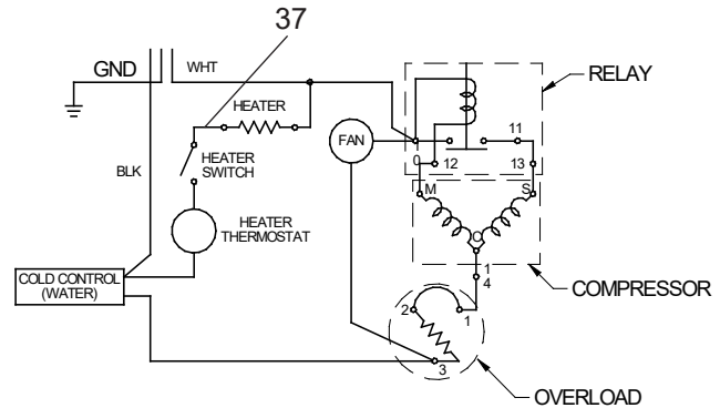
Wiring Diagram
