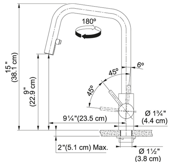
Dimensional Drawing
