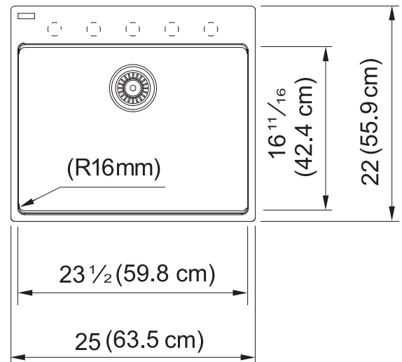
Dimensional Drawing
