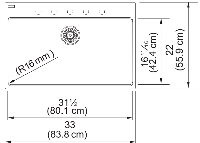
Dimensional Drawing
