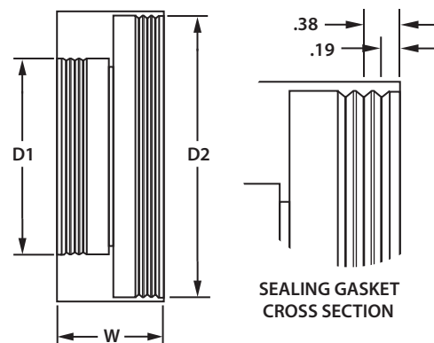
SEALING GASKET DETAILS
