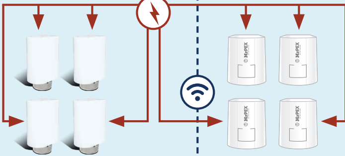
Self Balancing Wired Actuator
