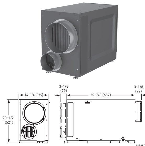
Fig. 1. Dimensions in in. (mm).
