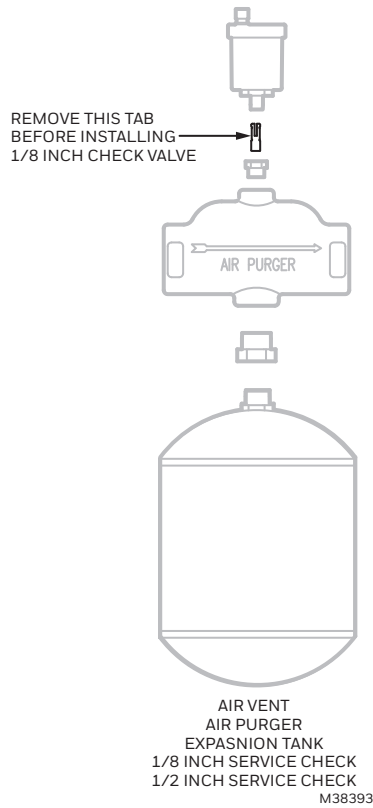
Fig. 1. Air Vent Air Purger Expansion Tank 1/8" service check; 1/2" service check.
