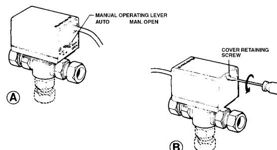
Fig. 1. Removing Cover
