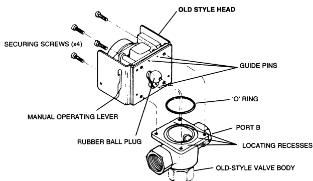
Fig. 2. Removing Powerheads
