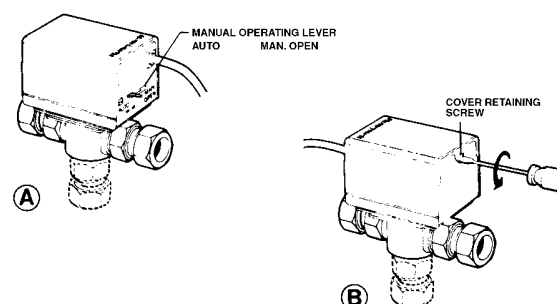
Fig. 1. Removing Cover
