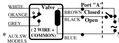
Fig. 7. Wiring color code for cable models for SPST controller. (Series 40 & 80)
