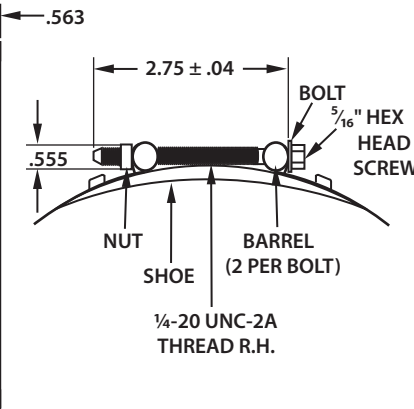
NUT & BOLT CLAMP DETAILS
