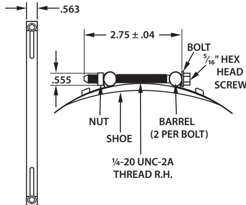
NUT & BOLT CLAMP DETAILS
