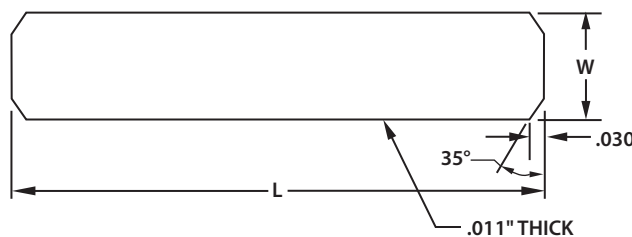
SHIELD DETAILS
