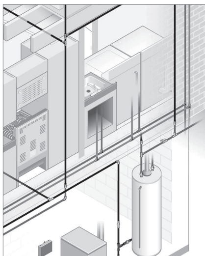
Branch-and-Tee Installation
