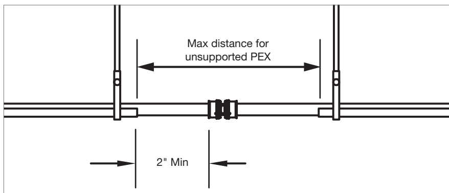
Fitting to tray / between trays
