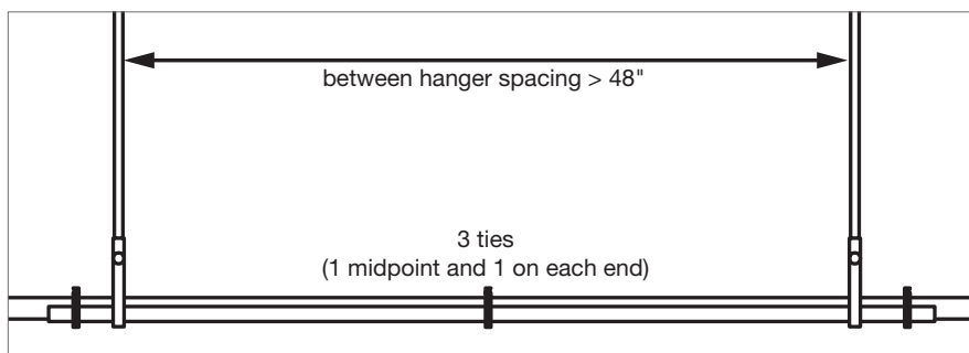
Tray strapping detail 3 ties
