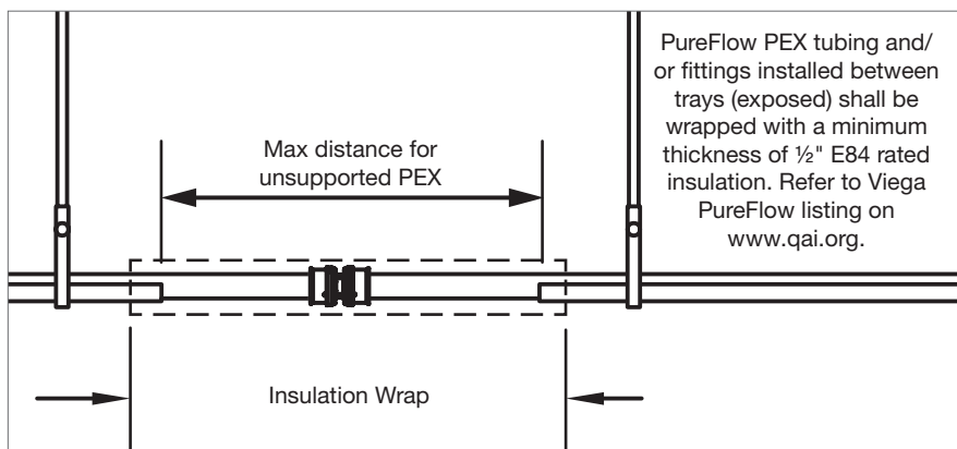
Plenum installation
