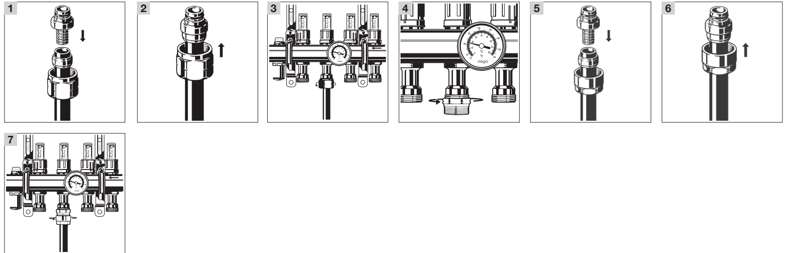
Model 1022SV
